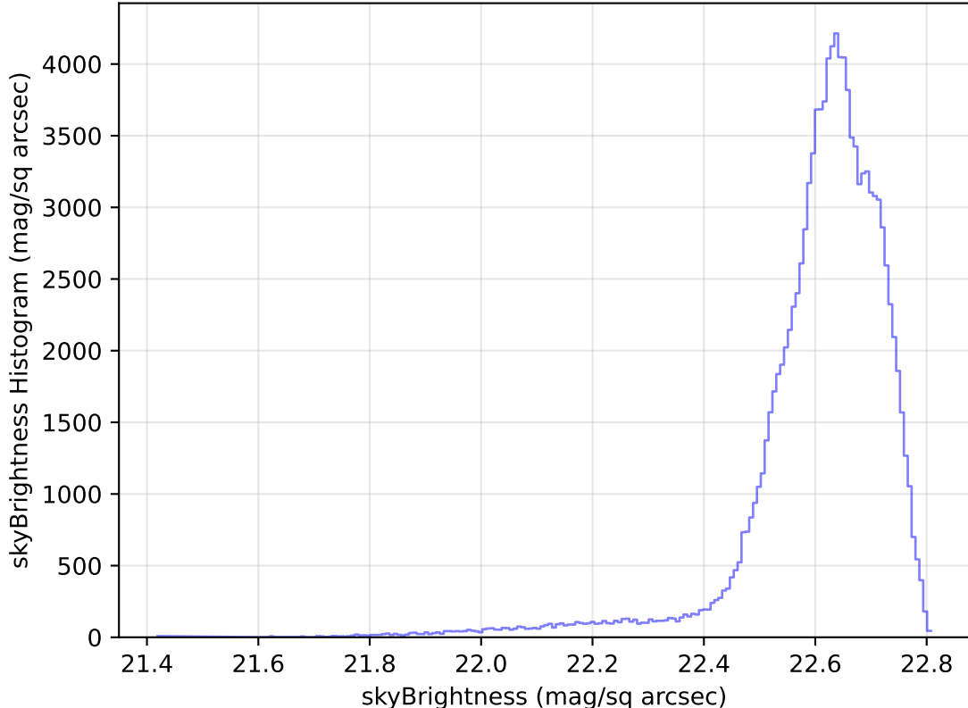
too_elab_heavy_r32_d3_griz_v3.4_10yrs All sky u band: skyBrightness Histogram
