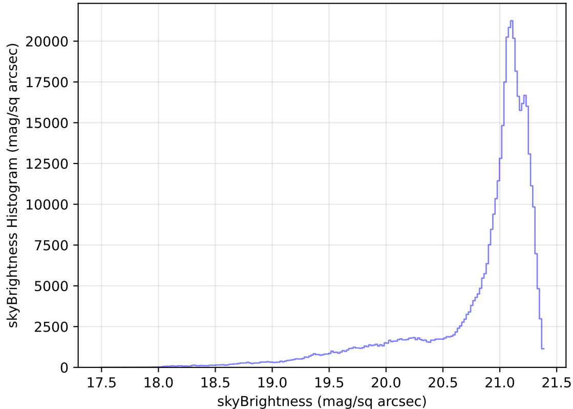
too_elab_heavy_r32_d3_griz_v3.4_10yrs All sky r band: skyBrightness Histogram
