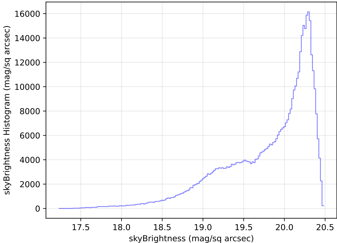
too_elab_heavy_r32_d3_griz_v3.4_10yrs All sky i band: skyBrightness Histogram
