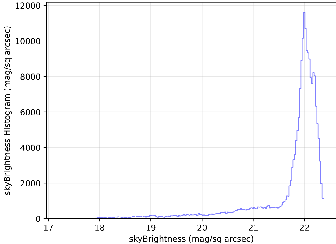
too_elab_heavy_r32_d3_griz_v3.4_10yrs All sky g band: skyBrightness Histogram
