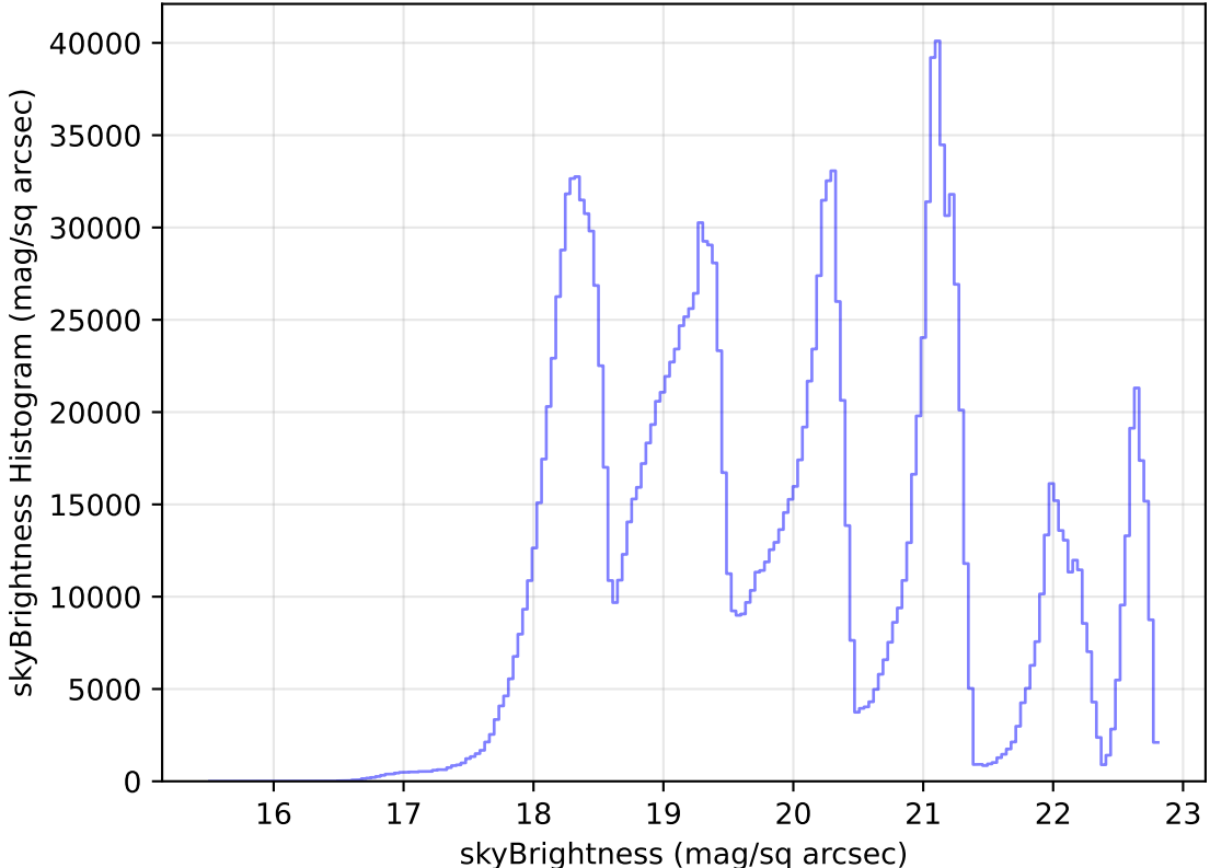
too_elab_heavy_r32_d3_griz_v3.4_10yrs All sky all bands: skyBrightness Histogram
