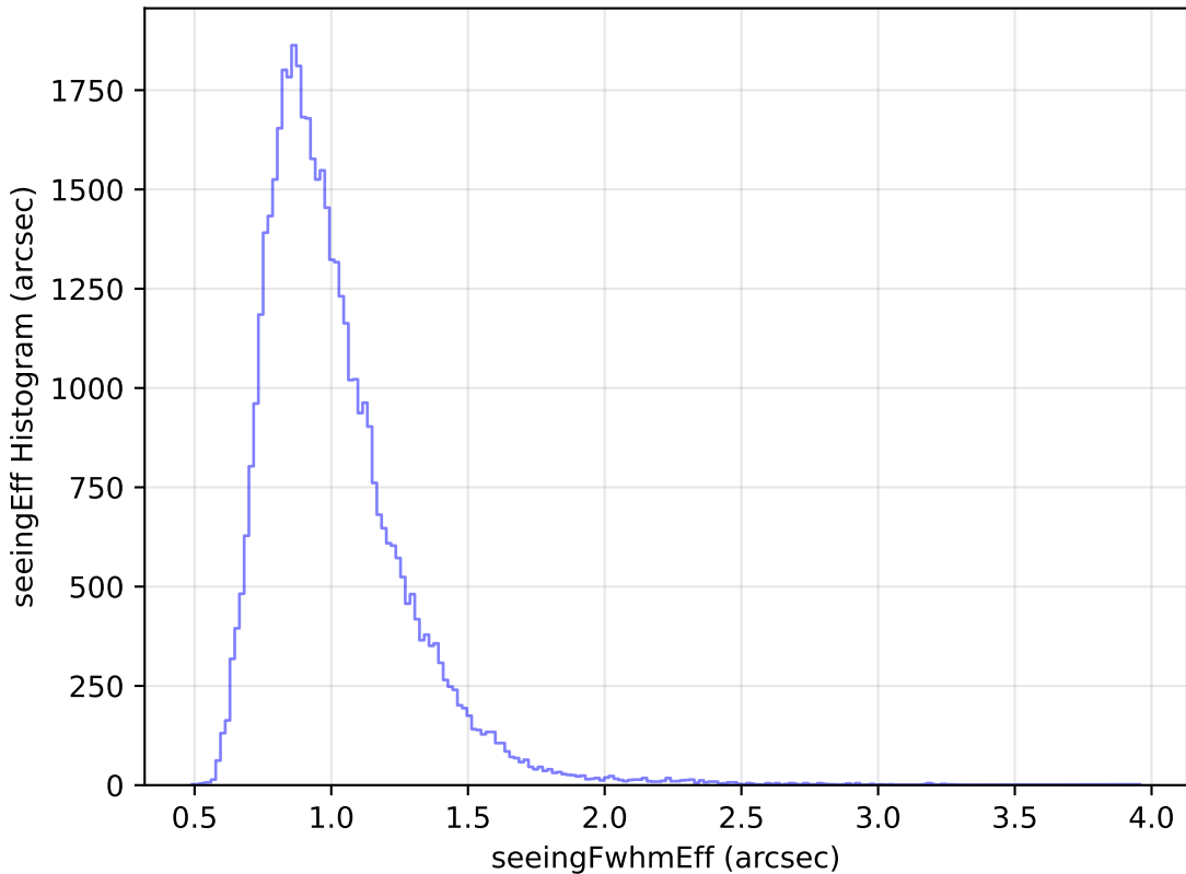
too_elab_heavy_r32_d3_griz_v3.4_10yrs Yr 1 y band: seeingEff Histogram
