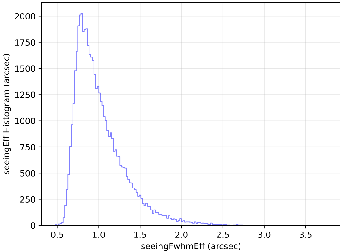
too_elab_heavy_r32_d3_griz_v3.4_10yrs Yr 1 r band: seeingEff Histogram
