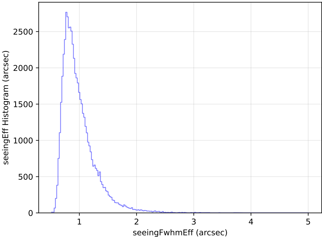
too_elab_heavy_r32_d3_griz_v3.4_10yrs Yr 1 i band: seeingEff Histogram
