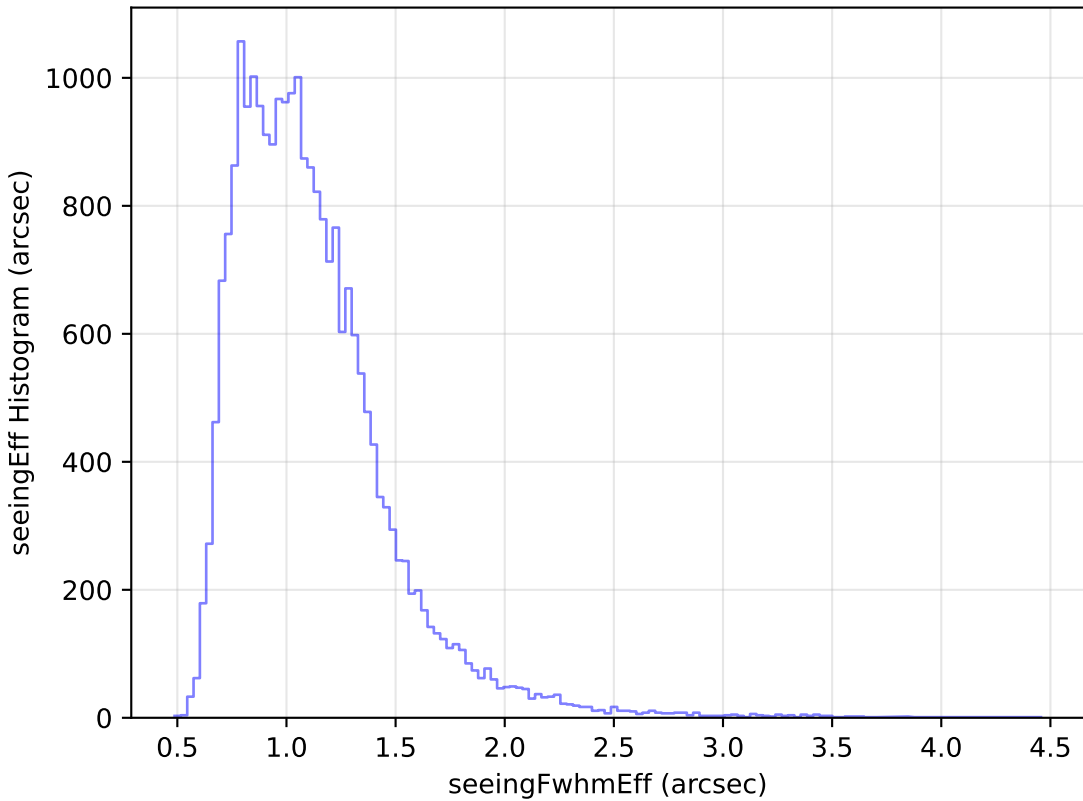
too_elab_heavy_r32_d3_griz_v3.4_10yrs Yr 1 g band: seeingEff Histogram
