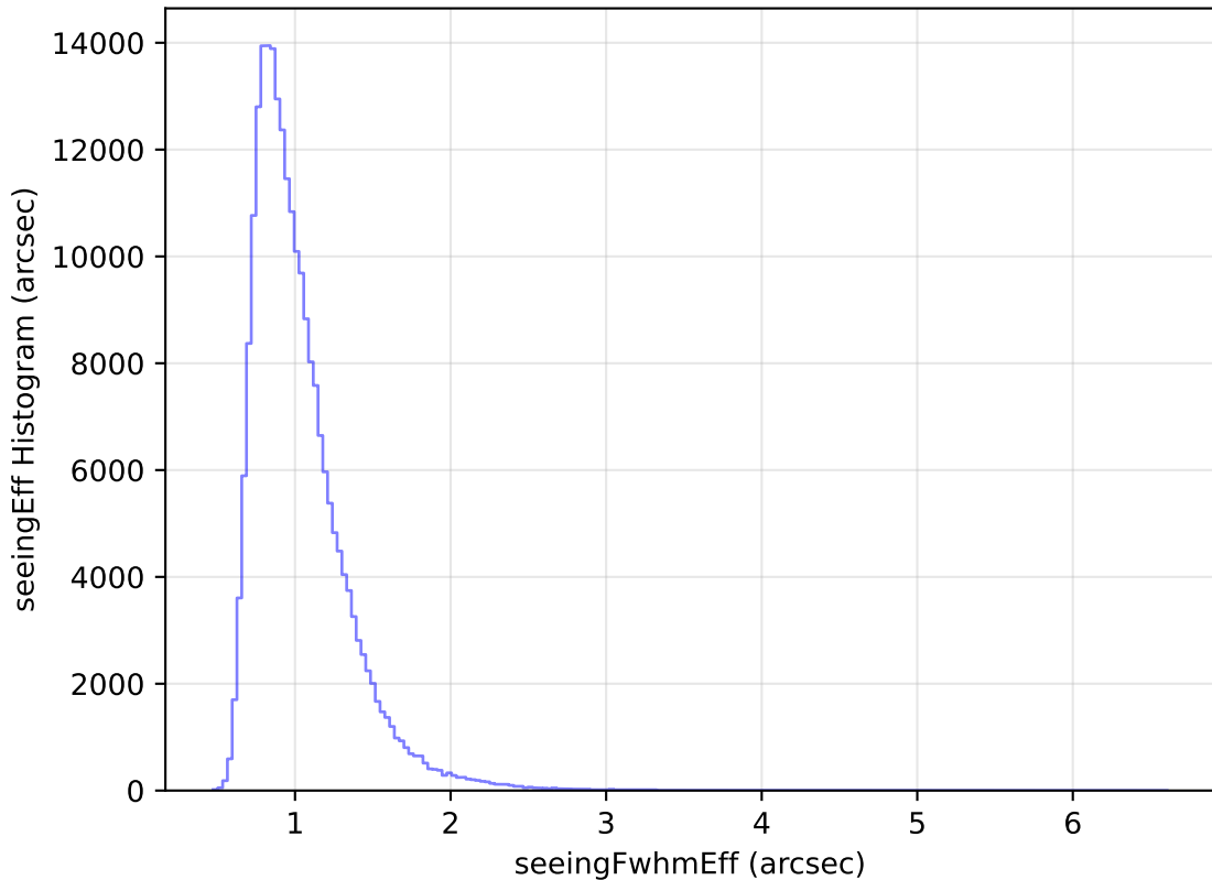
too_elab_heavy_r32_d3_griz_v3.4_10yrs Yr 1 all bands: seeingEff Histogram
