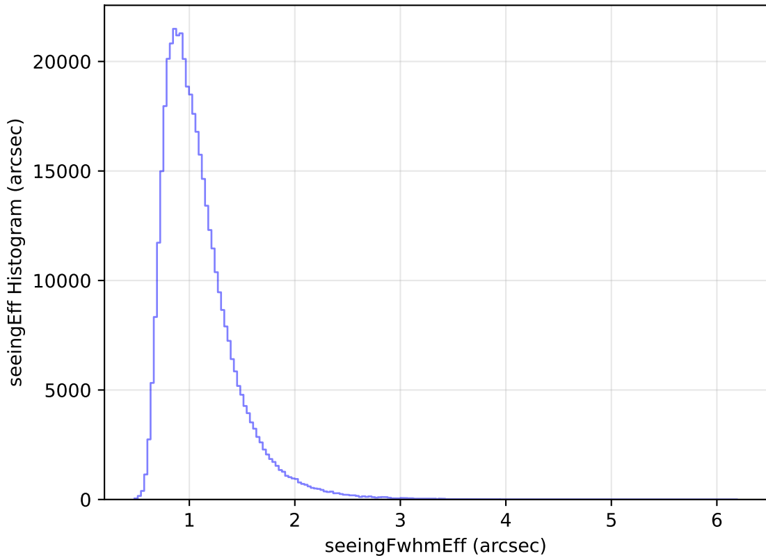
too_elab_heavy_r32_d3_griz_v3.4_10yrs WFD z band: seeingEff Histogram
