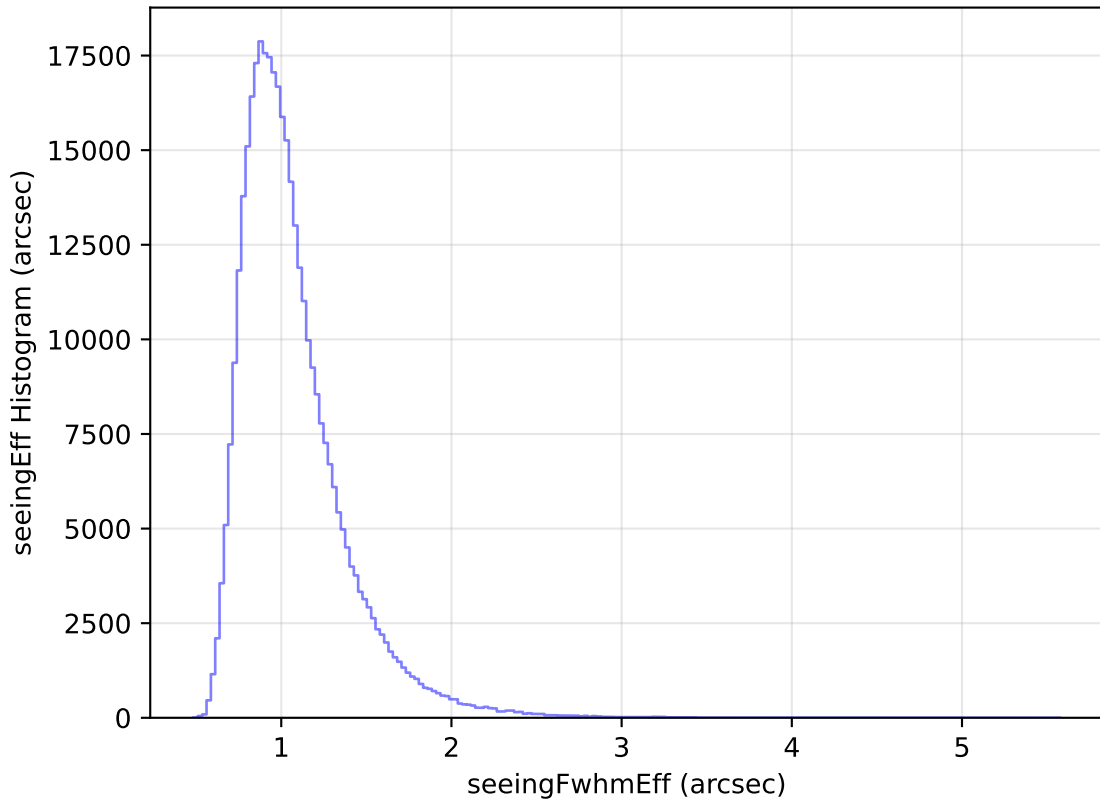
too_elab_heavy_r32_d3_griz_v3.4_10yrs WFD y band: seeingEff Histogram
