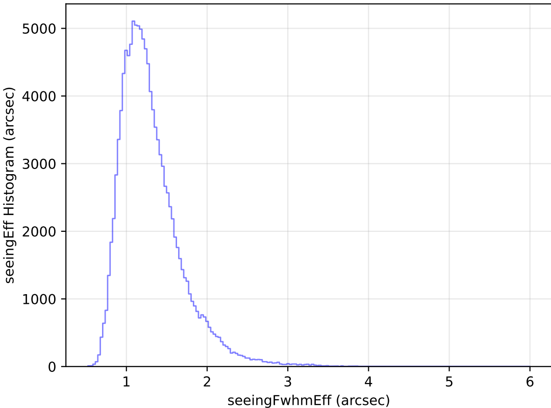
too_elab_heavy_r32_d3_griz_v3.4_10yrs WFD u band: seeingEff Histogram
