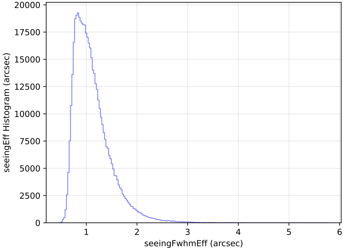
too_elab_heavy_r32_d3_griz_v3.4_10yrs WFD r band: seeingEff Histogram
