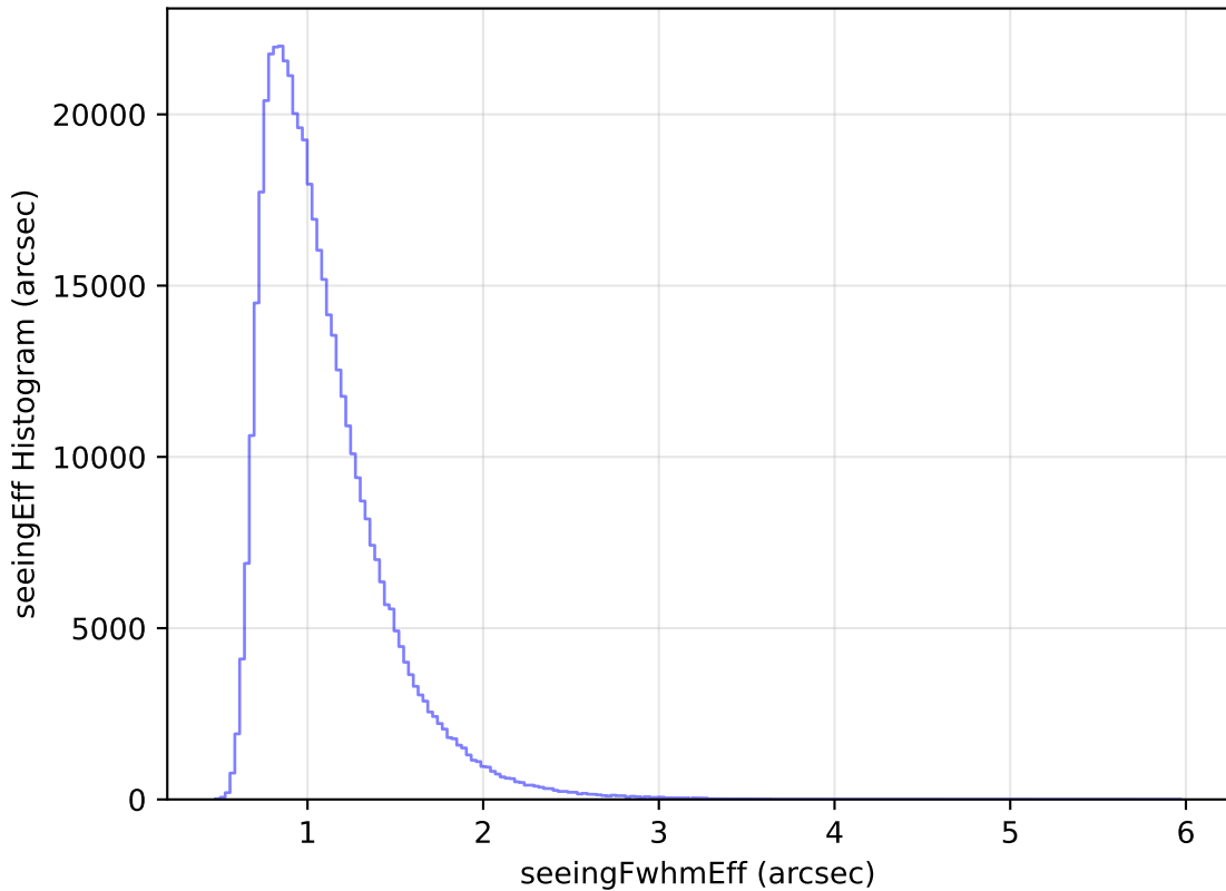
too_elab_heavy_r32_d3_griz_v3.4_10yrs WFD i band: seeingEff Histogram
