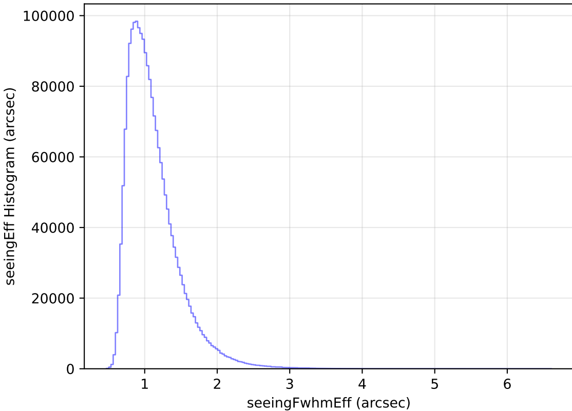
too_elab_heavy_r32_d3_griz_v3.4_10yrs WFD all bands: seeingEff Histogram
