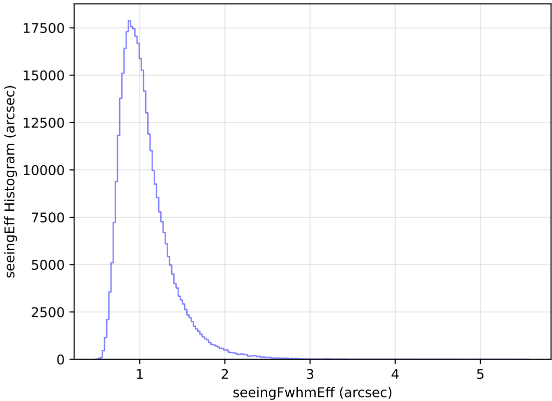
too_elab_heavy_r32_d3_griz_v3.4_10yrs All sky y band: seeingEff Histogram
