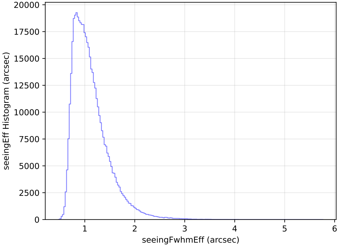
too_elab_heavy_r32_d3_griz_v3.4_10yrs All sky r band: seeingEff Histogram
