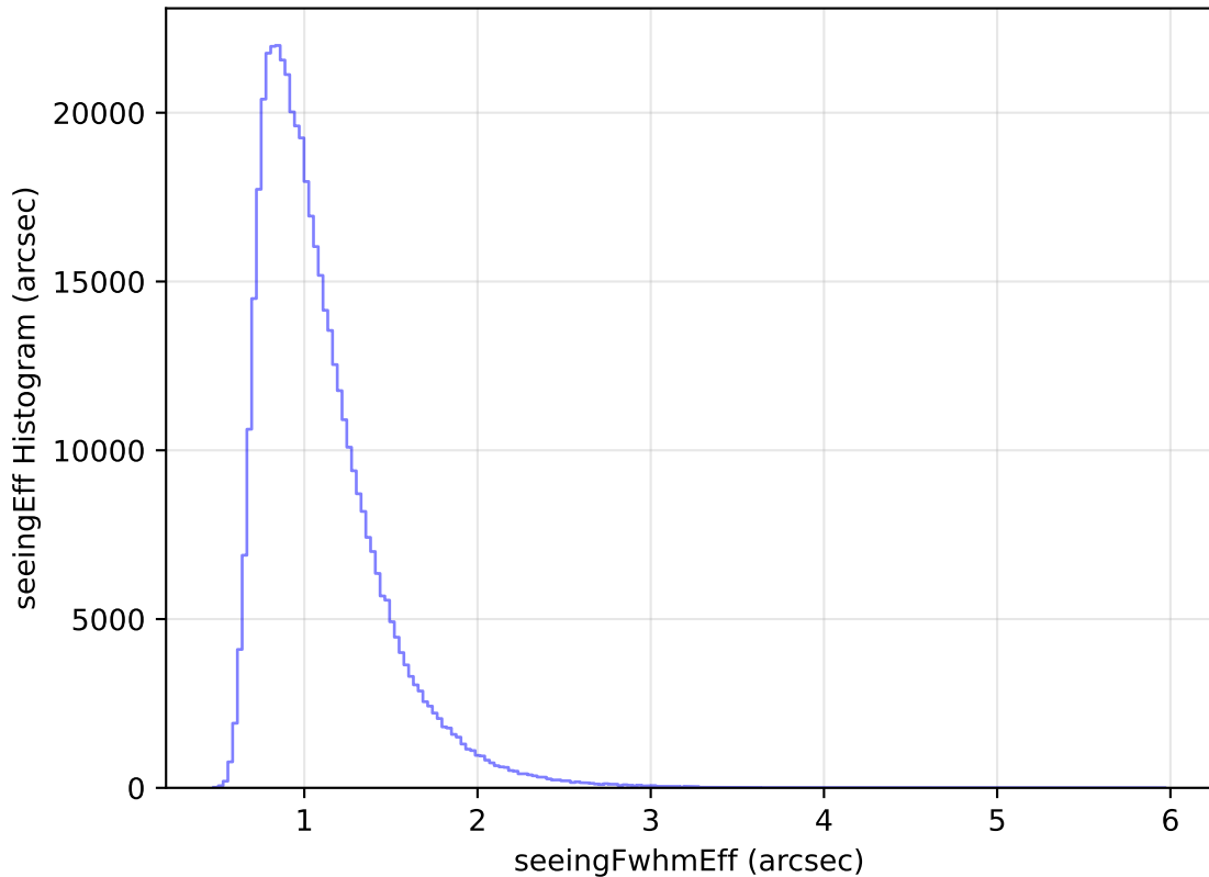
too_elab_heavy_r32_d3_griz_v3.4_10yrs All sky i band: seeingEff Histogram
