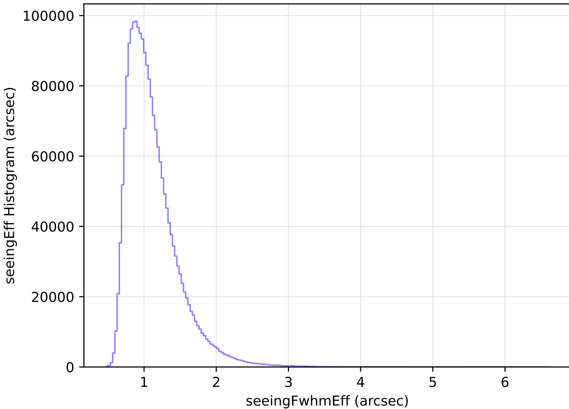
too_elab_heavy_r32_d3_griz_v3.4_10yrs All sky all bands: seeingEff Histogram
