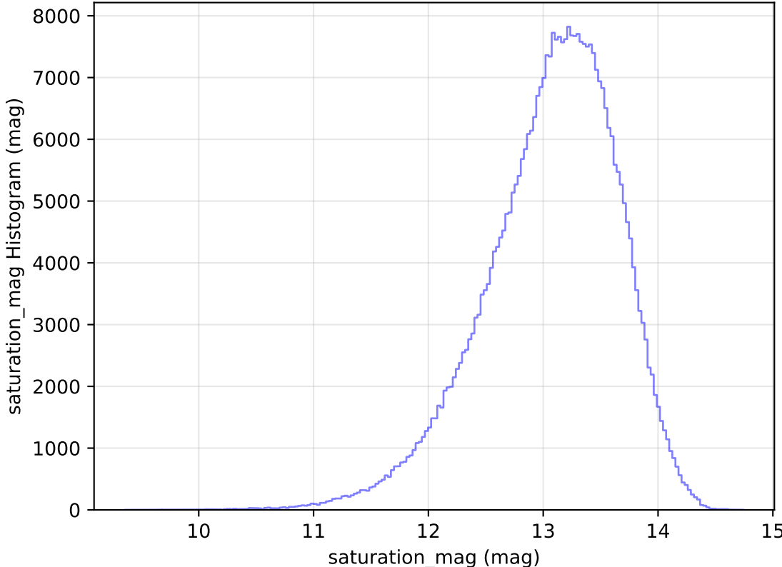
too_elab_heavy_r32_d3_griz_v3.4_10yrs WFD y band: saturation_mag Histogram
