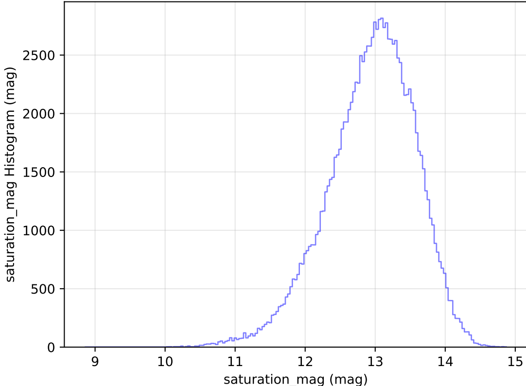
too_elab_heavy_r32_d3_griz_v3.4_10yrs WFD u band: saturation_mag Histogram
