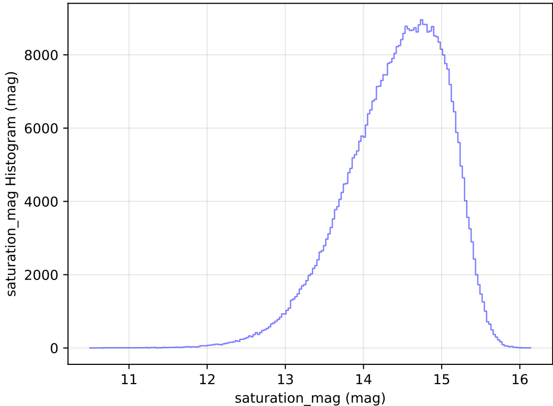
too_elab_heavy_r32_d3_griz_v3.4_10yrs WFD i band: saturation_mag Histogram
