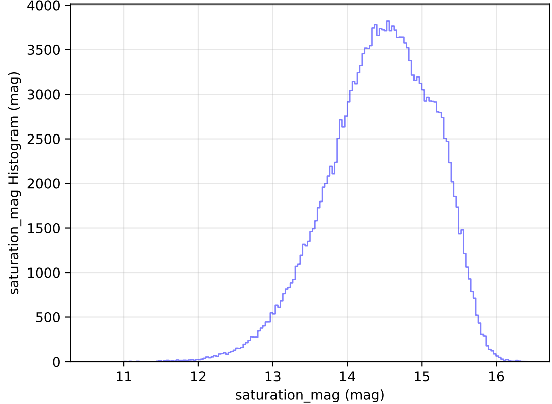
too_elab_heavy_r32_d3_griz_v3.4_10yrs WFD g band: saturation_mag Histogram
