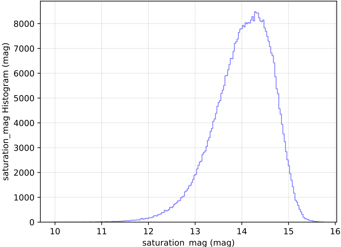
too_elab_heavy_r32_d3_griz_v3.4_10yrs All sky z band: saturation_mag Histogram
