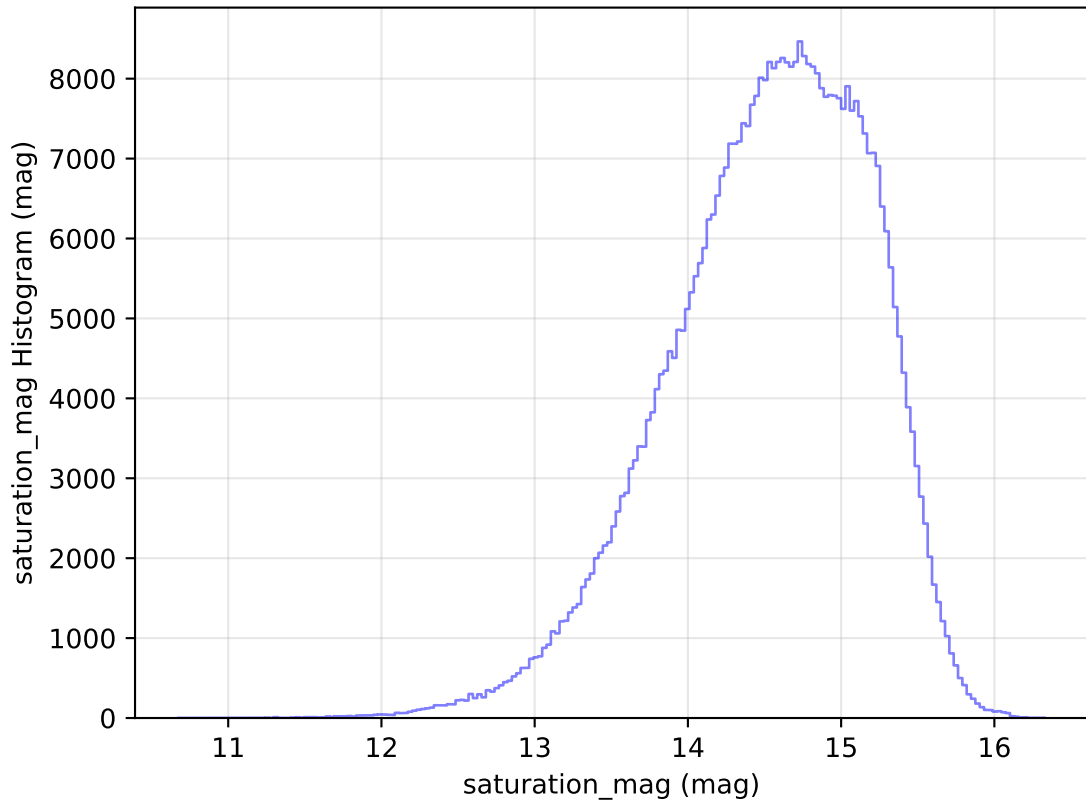
too_elab_heavy_r32_d3_griz_v3.4_10yrs All sky r band: saturation_mag Histogram
