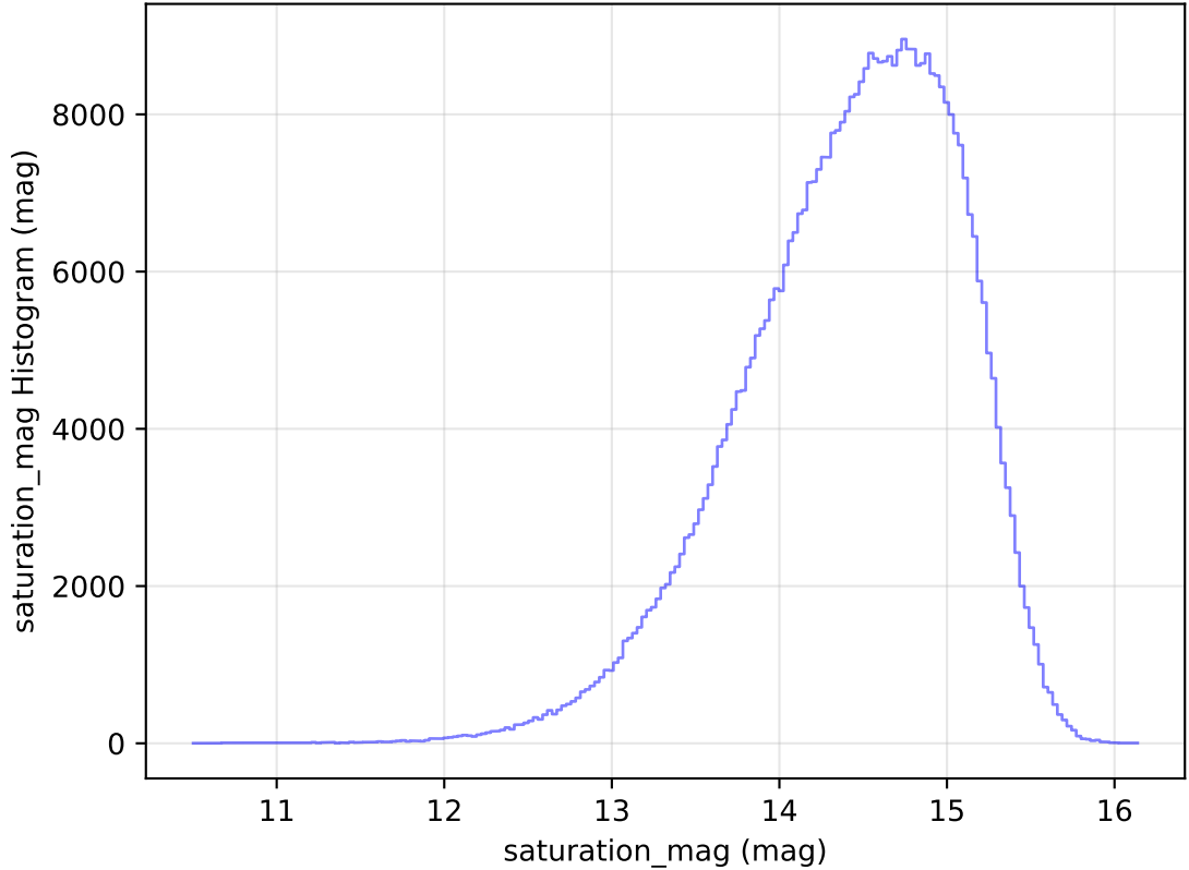
too_elab_heavy_r32_d3_griz_v3.4_10yrs All sky i band: saturation_mag Histogram
