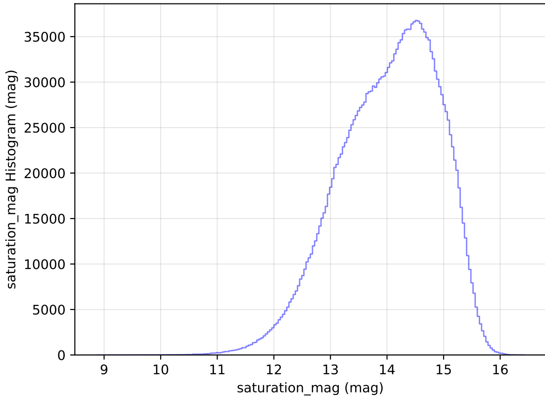
too_elab_heavy_r32_d3_griz_v3.4_10yrs All sky all bands: saturation_mag Histogram
