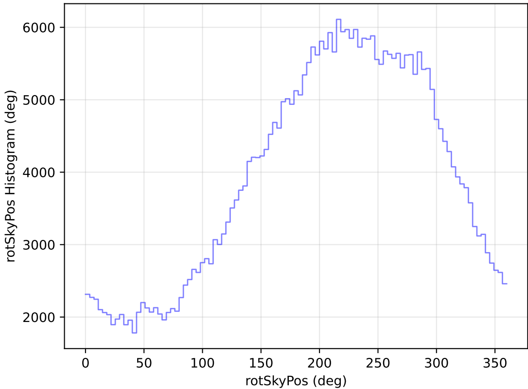
too_elab_heavy_r32_d3_griz_v3.4_10yrs WFD y band: rotSkyPos Histogram
