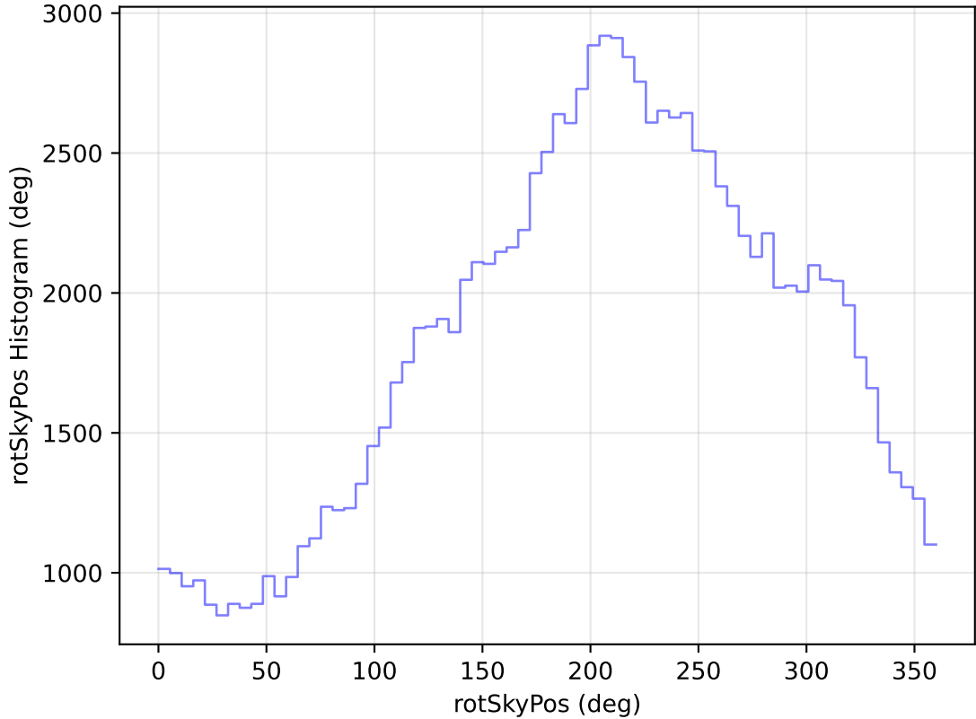
too_elab_heavy_r32_d3_griz_v3.4_10yrs WFD u band: rotSkyPos Histogram
