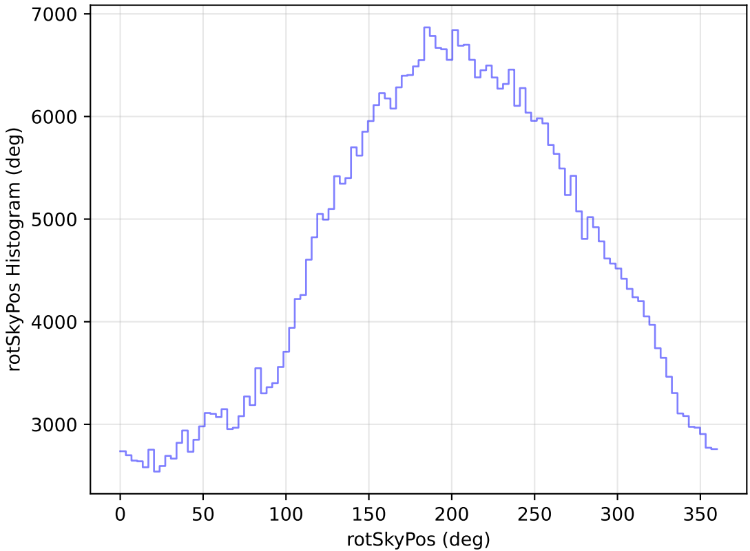
too_elab_heavy_r32_d3_griz_v3.4_10yrs WFD r band: rotSkyPos Histogram
