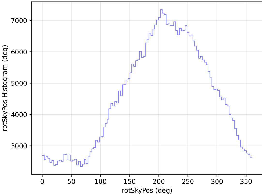
too_elab_heavy_r32_d3_griz_v3.4_10yrs WFD i band: rotSkyPos Histogram
