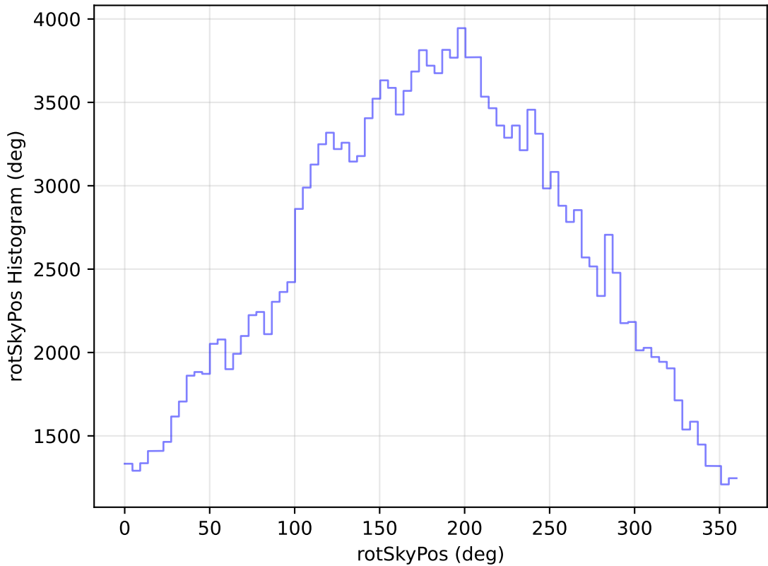
too_elab_heavy_r32_d3_griz_v3.4_10yrs WFD g band: rotSkyPos Histogram
