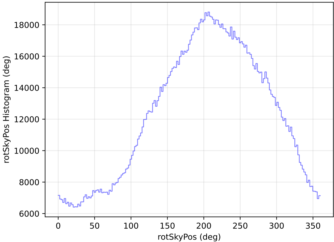
too_elab_heavy_r32_d3_griz_v3.4_10yrs WFD all bands: rotSkyPos Histogram
