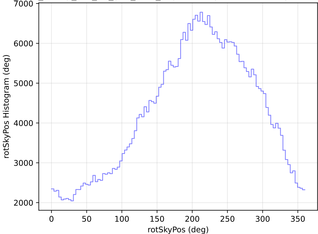
too_elab_heavy_r32_d3_griz_v3.4_10yrs All sky z band: rotSkyPos Histogram
