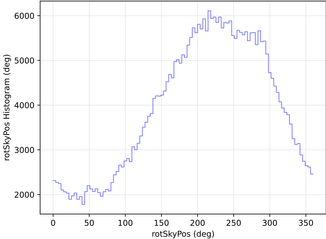
too_elab_heavy_r32_d3_griz_v3.4_10yrs All sky y band: rotSkyPos Histogram
