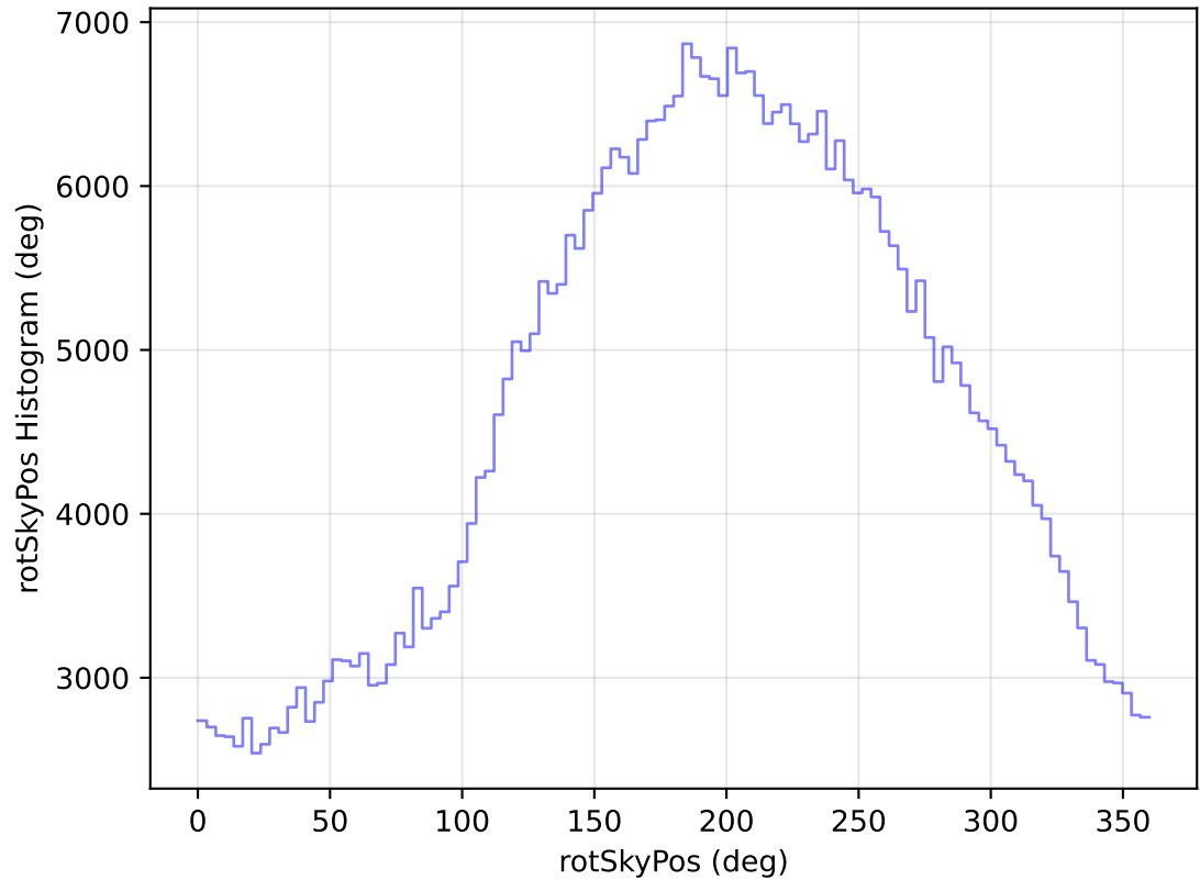
too_elab_heavy_r32_d3_griz_v3.4_10yrs All sky r band: rotSkyPos Histogram
