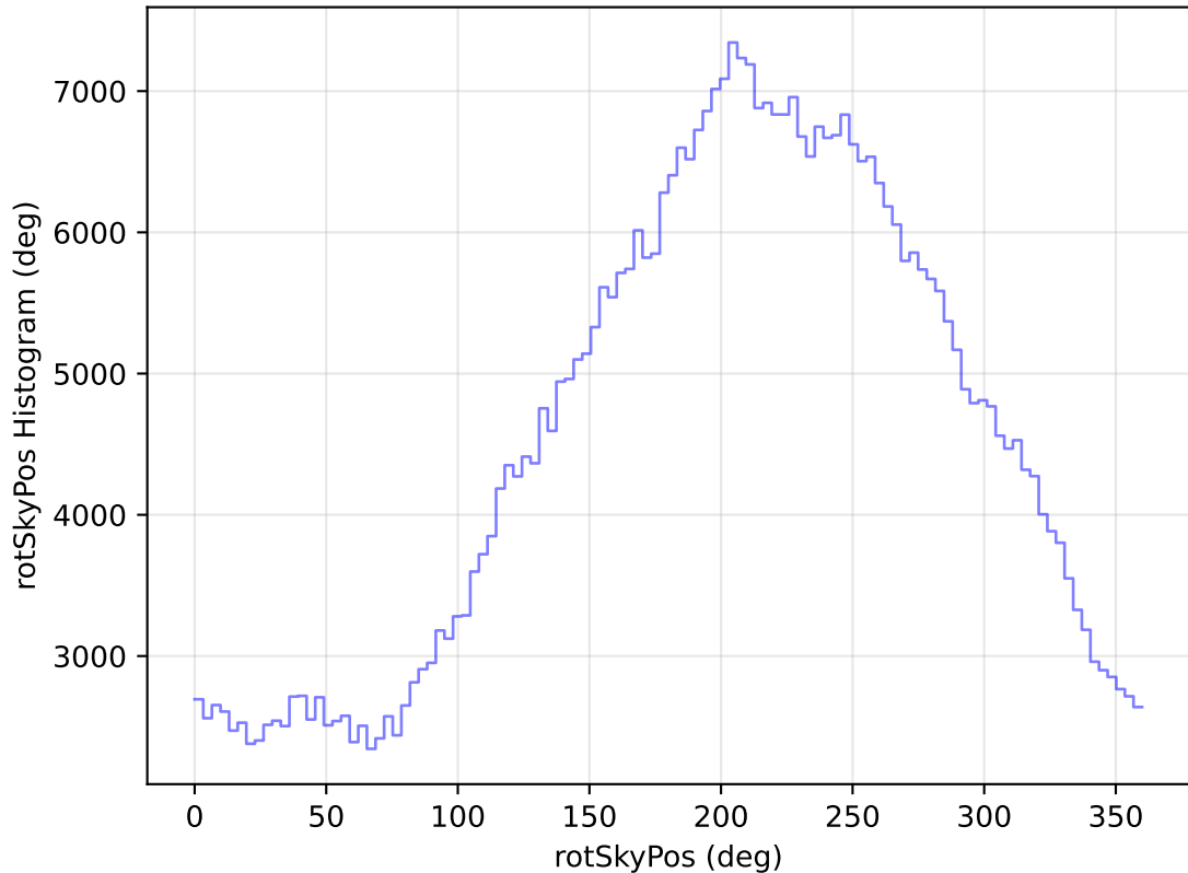
too_elab_heavy_r32_d3_griz_v3.4_10yrs All sky i band: rotSkyPos Histogram
