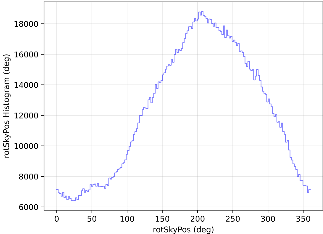
too_elab_heavy_r32_d3_griz_v3.4_10yrs All sky all bands: rotSkyPos Histogram
