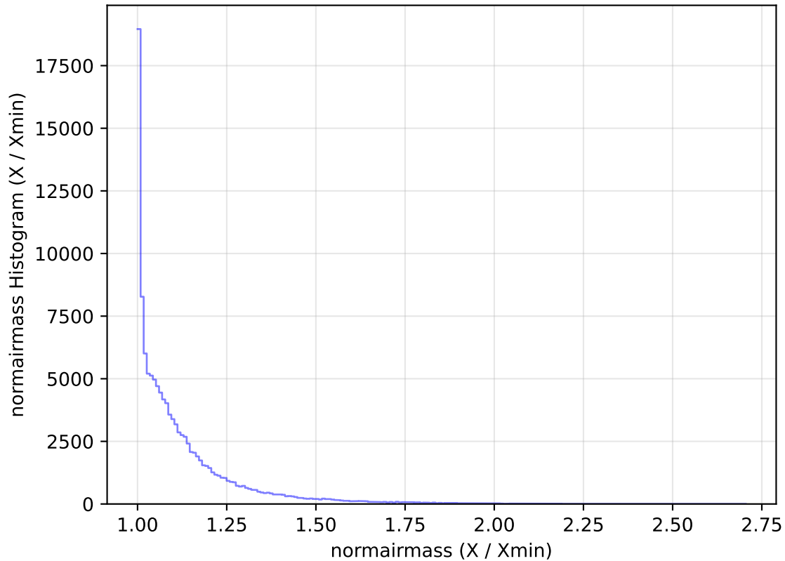
too_elab_heavy_r32_d3_griz_v3.4_10yrs WFD u band: normairmass Histogram
