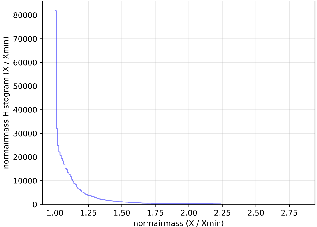
too_elab_heavy_r32_d3_griz_v3.4_10yrs WFD r band: normairmass Histogram
