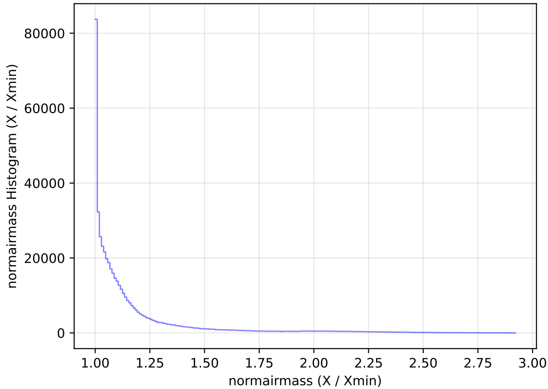
too_elab_heavy_r32_d3_griz_v3.4_10yrs WFD i band: normairmass Histogram
