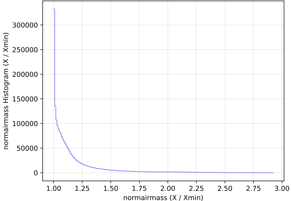
too_elab_heavy_r32_d3_griz_v3.4_10yrs WFD all bands: normairmass Histogram
