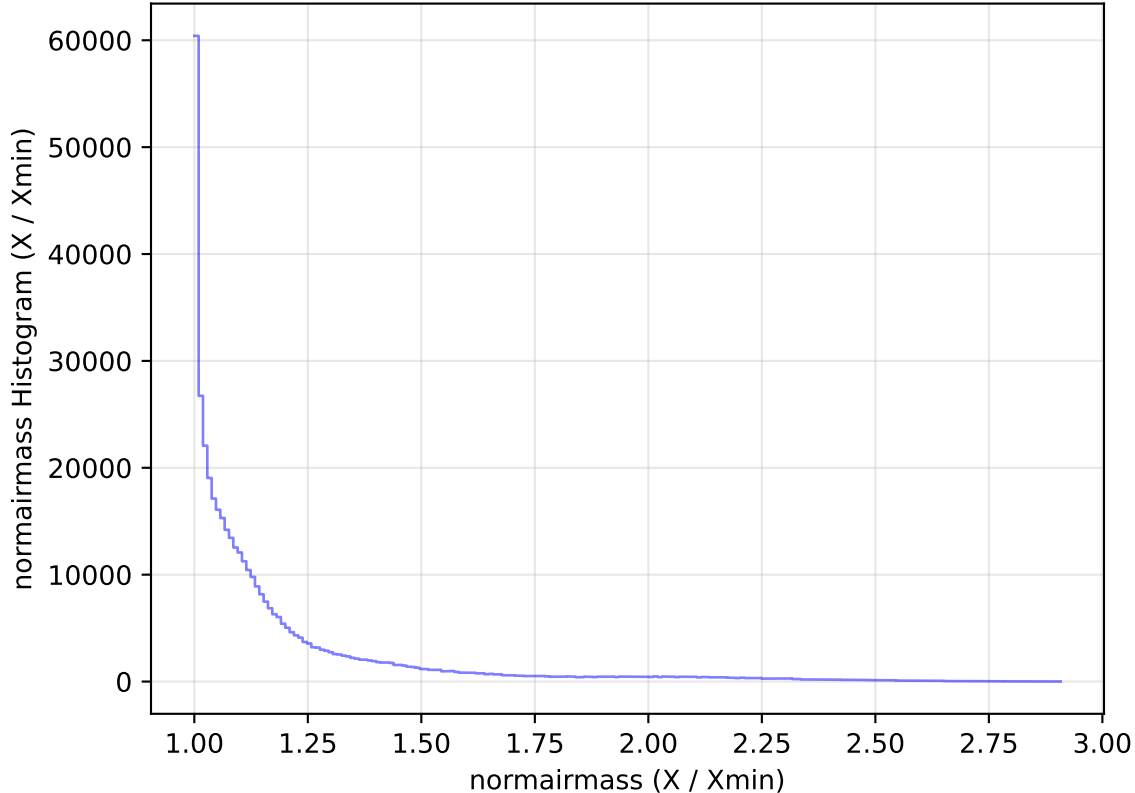
too_elab_heavy_r32_d3_griz_v3.4_10yrs All sky z band: normairmass Histogram
