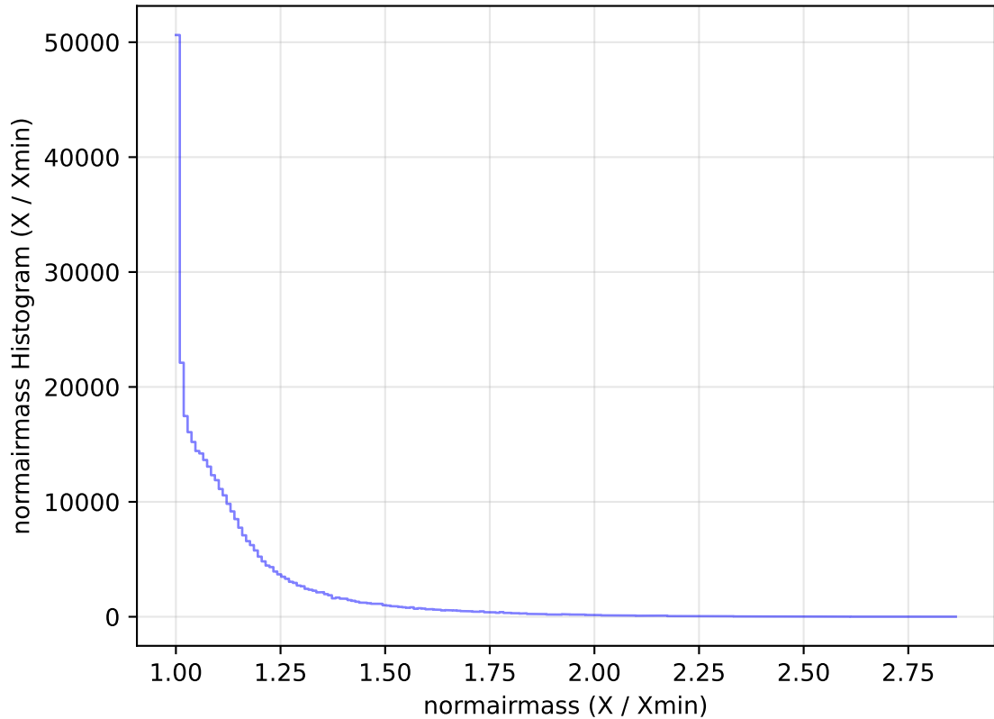
too_elab_heavy_r32_d3_griz_v3.4_10yrs All sky y band: normairmass Histogram
