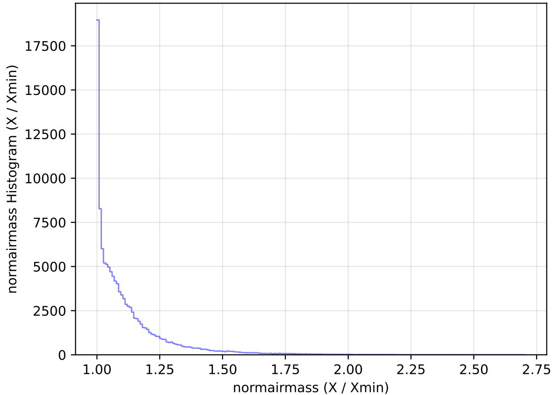
too_elab_heavy_r32_d3_griz_v3.4_10yrs All sky u band: normairmass Histogram
