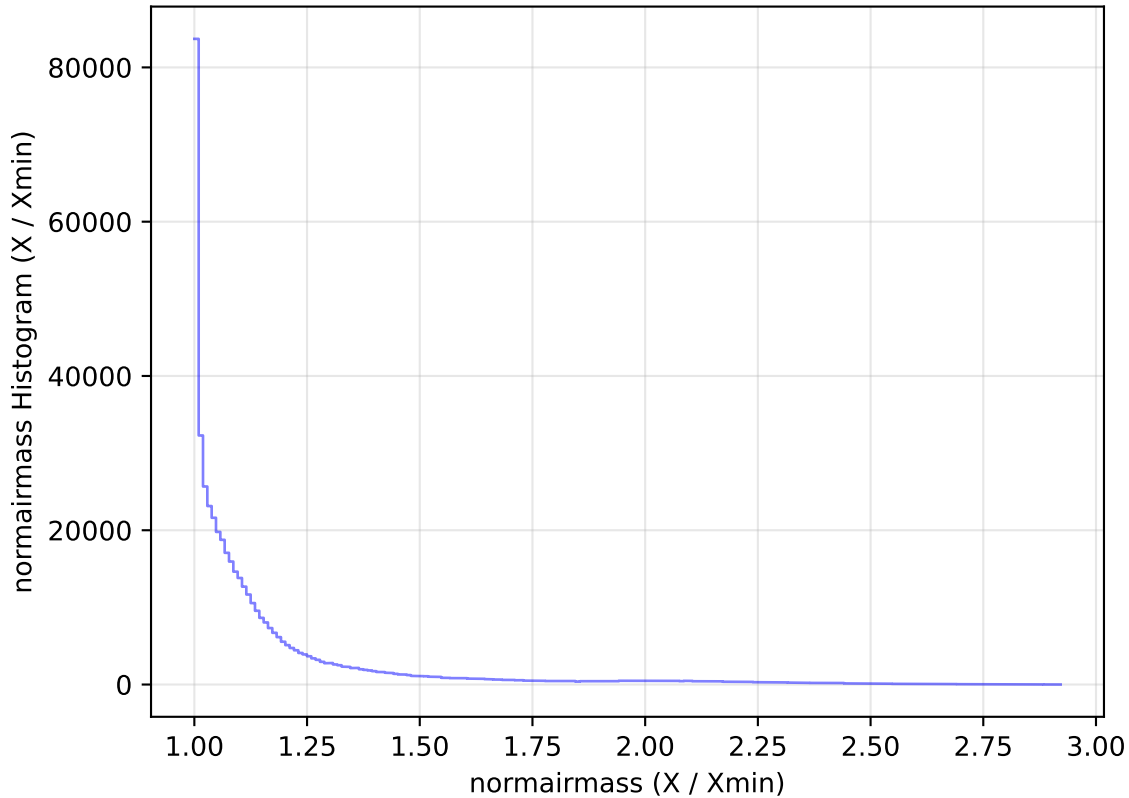
too_elab_heavy_r32_d3_griz_v3.4_10yrs All sky i band: normairmass Histogram
