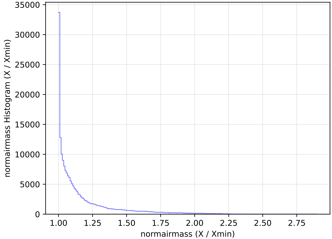
too_elab_heavy_r32_d3_griz_v3.4_10yrs All sky g band: normairmass Histogram
