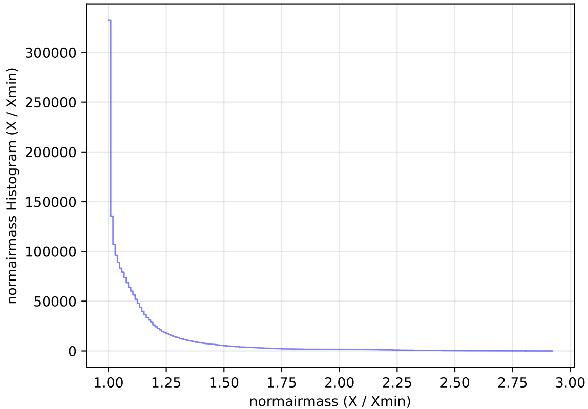
too_elab_heavy_r32_d3_griz_v3.4_10yrs All sky all bands: normairmass Histogram
