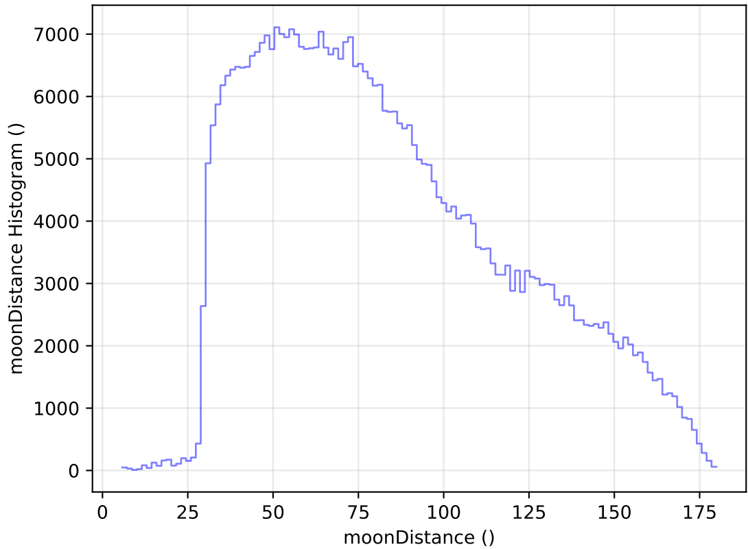
too_elab_heavy_r32_d3_griz_v3.4_10yrs WFD z band: moonDistance Histogram
